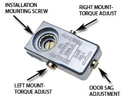
Figure 20 TorqueMaster Assembly
