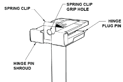
Figure 13 Hinge Pin Assembly
