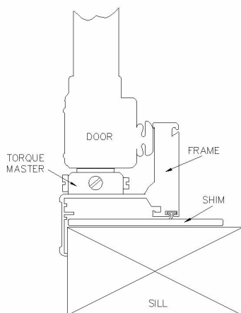
Figure 1 Anthony Door and Frame Cross-Section
