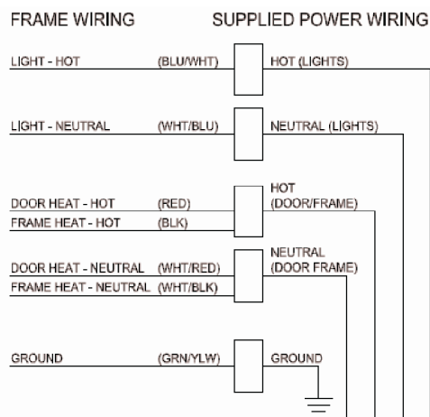
Figure 4 Wiring Diagram
